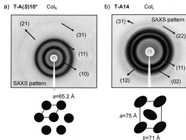
Figure 2. SAXS patterns with indexing of a) the Col h mesophase of complex T-A(S)10* , where a is the lattice parameter of the hexagonal arrangement of the chiral complex, and b) the Col r mesophase of complex T-A14 , where a and b are the lattice parameters of the rectangular arrangement of the achiral complex. Both patterns were recorded at room temperature after cooling from the isotropic liquid.
