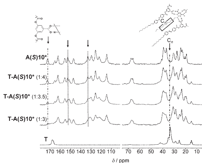
Figure 1. ^{13}\text{C} CPMAS NMR spectra of T , A(S)10* , and mixtures of T and A(S)10* with different proportions of acid. Arrows indicate the most meaningful shift differences indicating the presence or absence of free acid.
