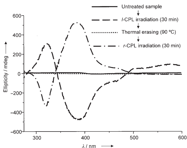
Figure 4. CD spectra corresponding to a l -CPL irradiation/thermal erasing/ r -CPL irradiation cycle for a cast film of complex T-A14 . The irradiation times are given with respect to the previous irradiation step.
