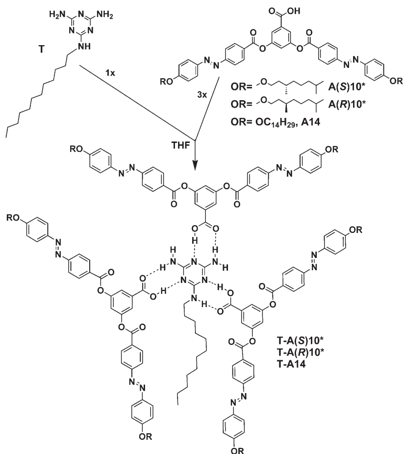
Scheme 1. Synthesis of hydrogen-bonded complexes that incorporate azobenzene groups in each of the arms of the V-shaped acid.
