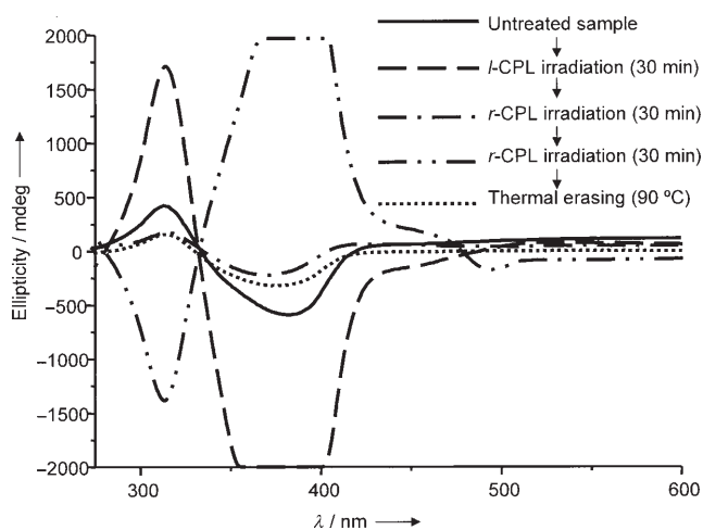
Figure 3. CD spectra corresponding to successive irradiation of a cast film of complex T-(R)A10* with l -CPL and r -CPL at room temperature. The irradiation times are given with respect to the previous irradiation step.
